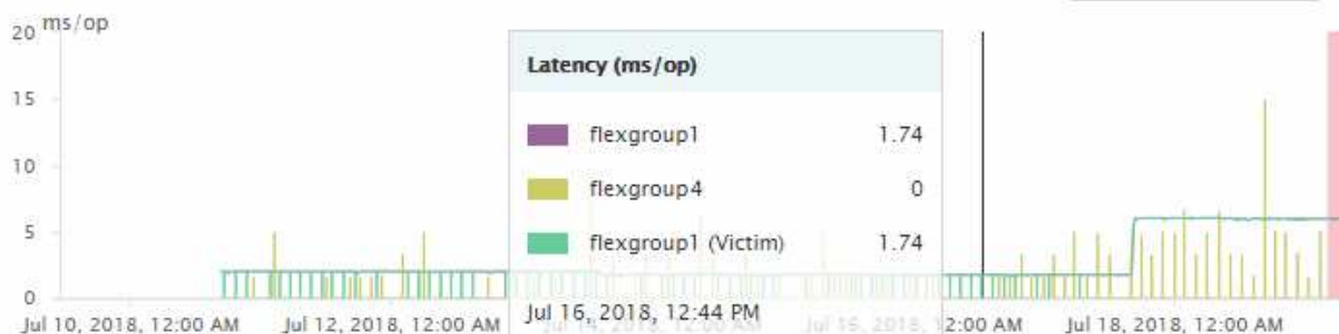
Workload Latency
