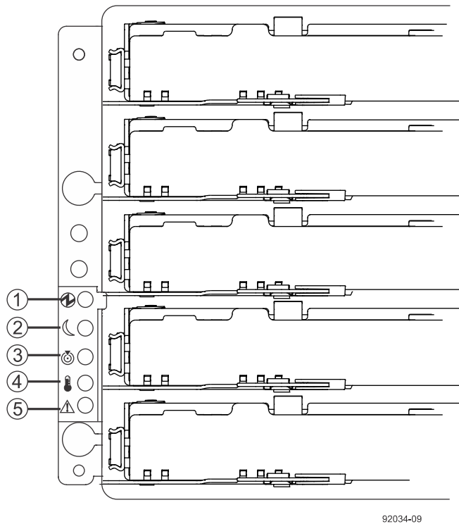
Figure 1. LEDs on the Left End Cap of the DE6600 Drive Tray – Front View with the Bezel Removed
