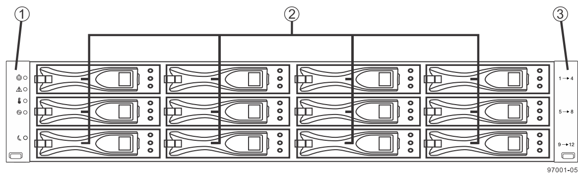
E5612 controller-drive tray – front view
