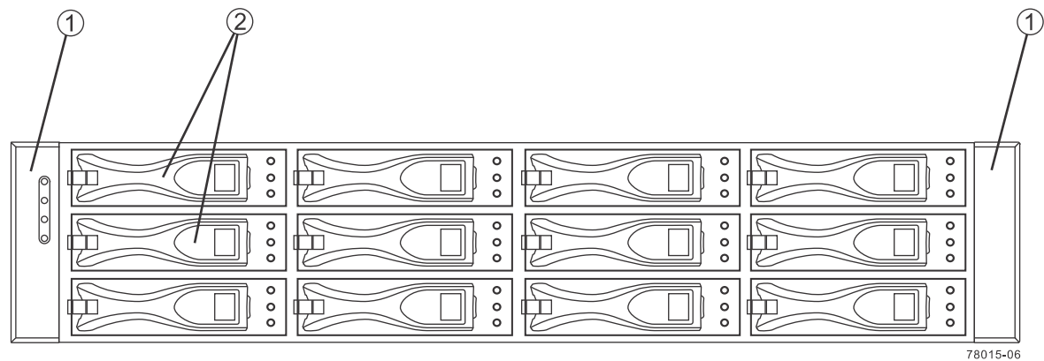
E2612 controller-drive tray with 12 drives – front view
