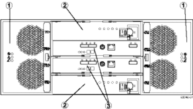
DE6600 drive tray - rear view
