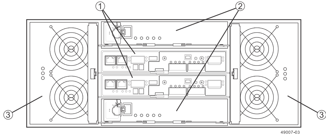
E2760 controller-drive tray – rear view
