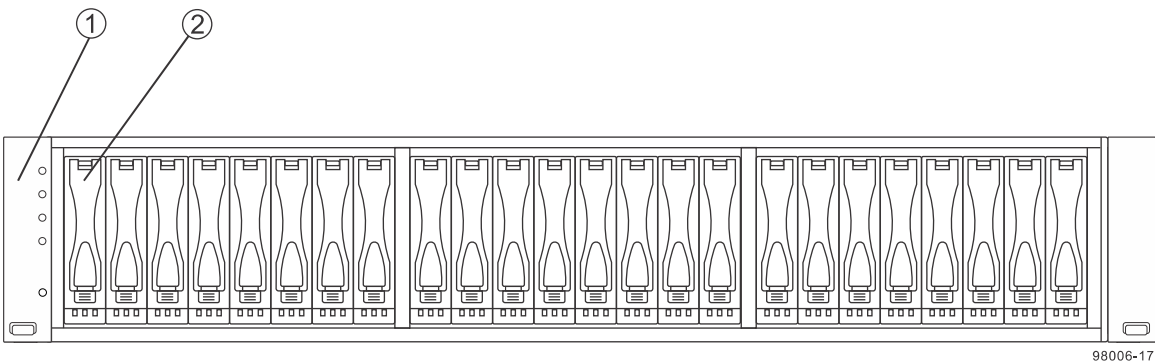
E5424 controller-drive tray or EF540 flash array with 24 drives – front view
