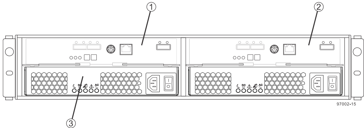
DE1600 drive tray – rear view
