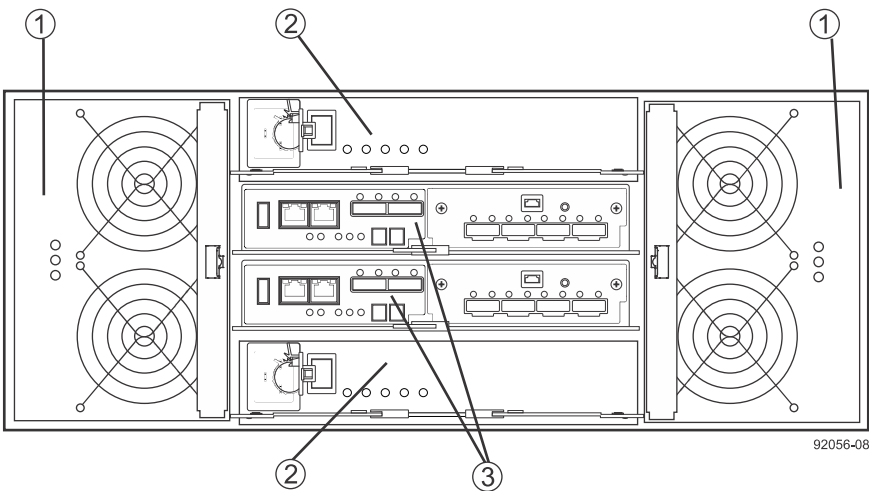
E5560 controller-drive tray – rear view
