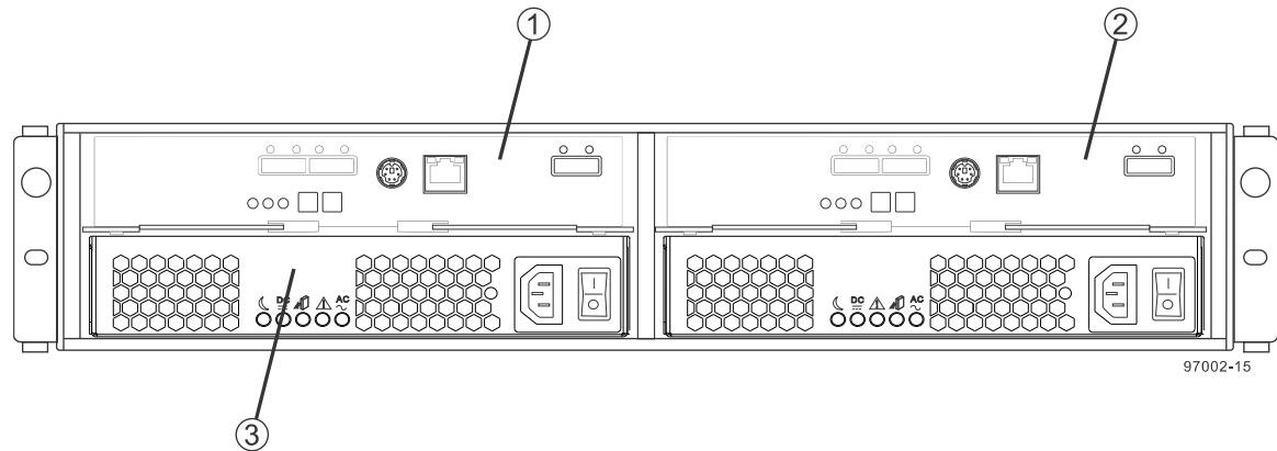
DE5600 drive tray – rear view
