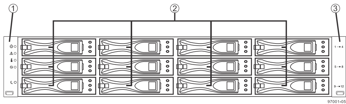
E5512 controller-drive tray with 12 drives – front view
