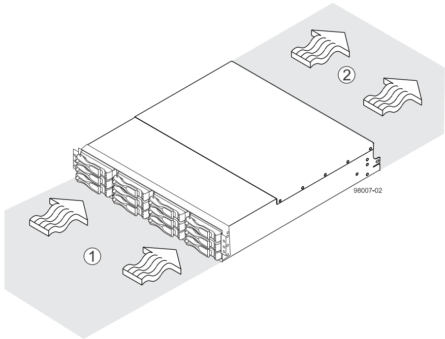
Airflow through the E2612 controller-drive tray – front view
