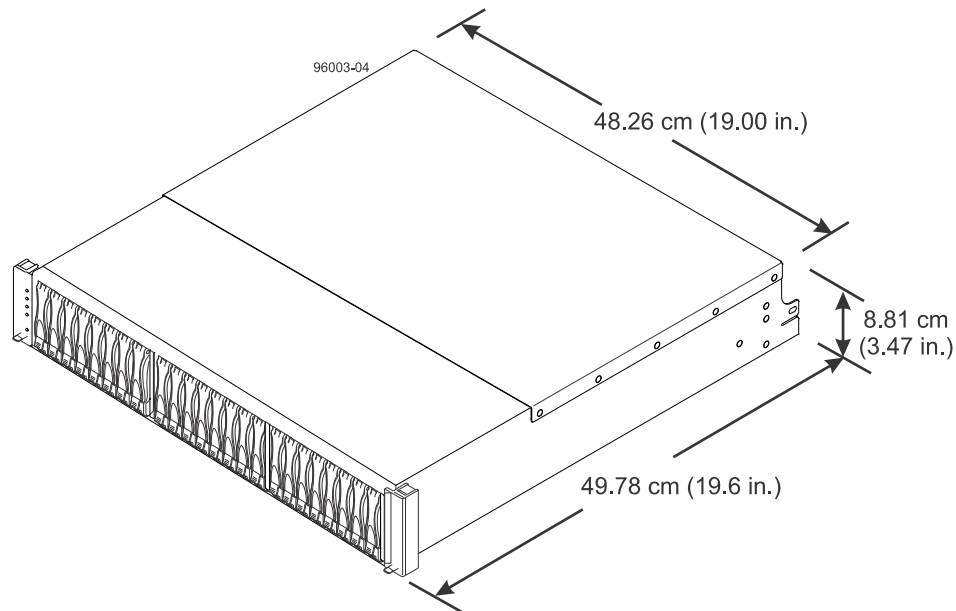
Dimensions of the E5624 controller drive tray and the EF560 flash array – front view
