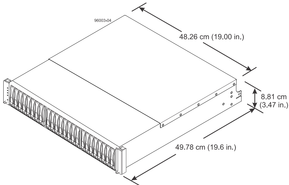
Dimensions of the E2724 controller-drive tray – front view
