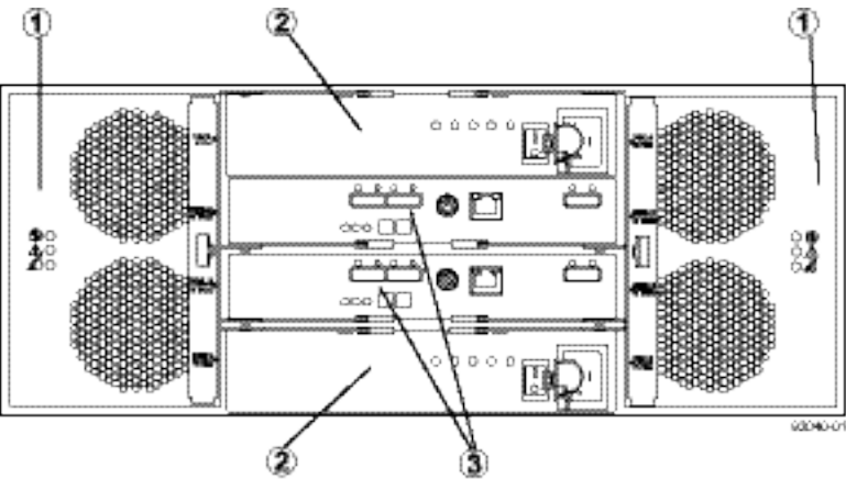
E2660 controller-drive tray – rear view
