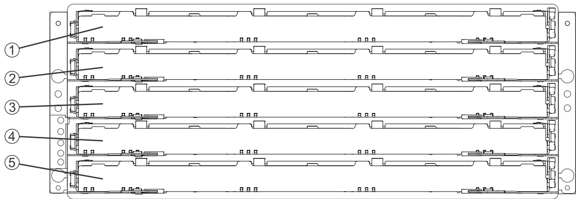
DE6600 drive tray – front view with bezel removed
