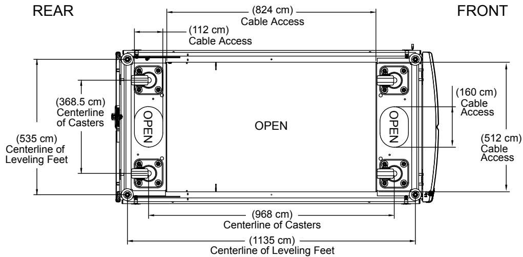
BOTTEM VIEW OF CABINET
