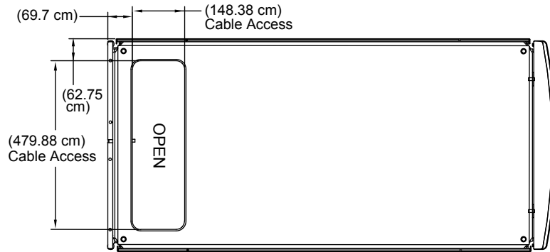
TOP VIEW OF CABINET
