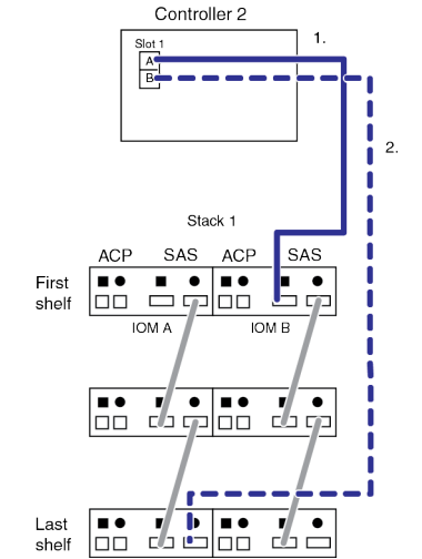
Single-controller-dual-path configuration
