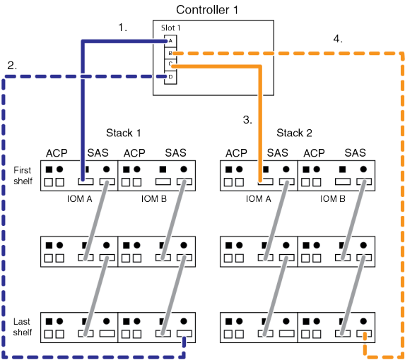
Single-controller-dual-path configuration
