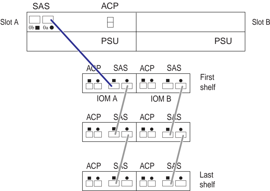
Single-controller-single-path configuration
