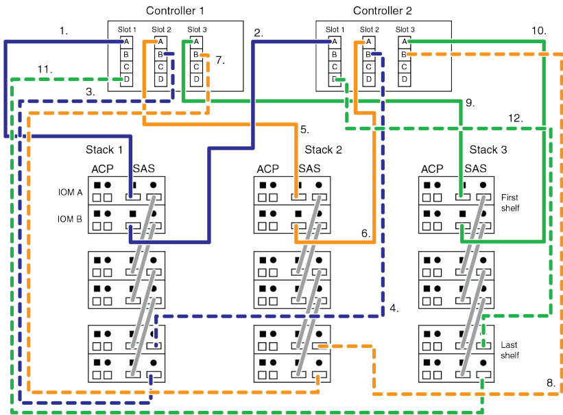
Multipath HA configuration
