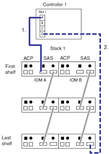
Single-controller-dual-path configuration
