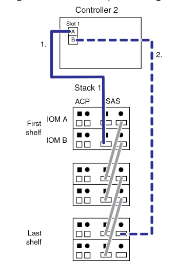
Single-controller-dual-path configuration
