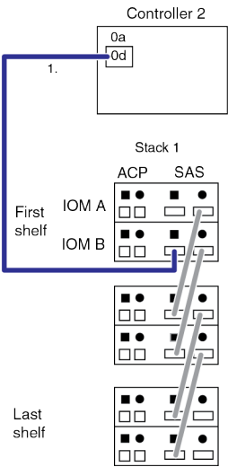
Single-controller-single-path configuration
