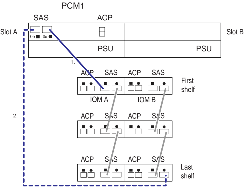
Single-controller-dual-path configuration
