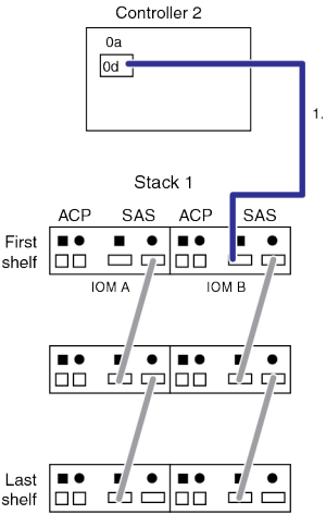
Single-controller-single-path configuration
