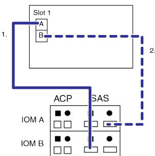
Single-controller-dual-path configuration Controller 2
