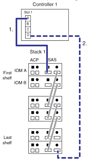
Single-controller-dual-path configuration
