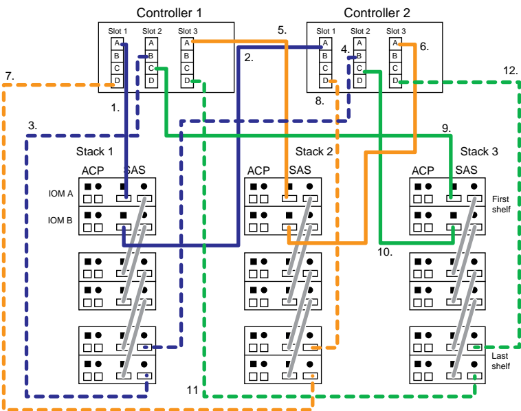
Multipath HA configuration
