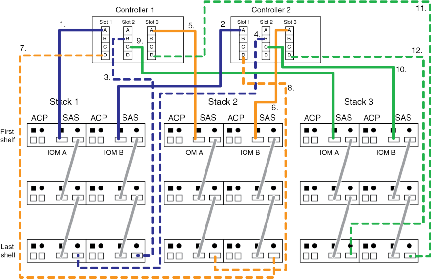
Multipath HA configuration
