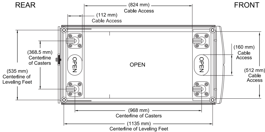
BOTTEM VIEW OF CABINET
