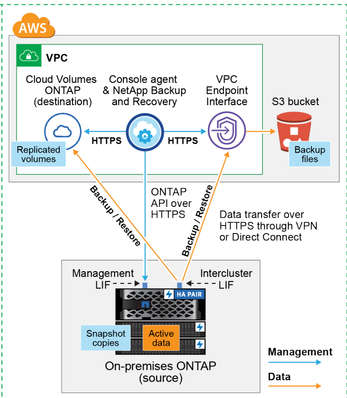
Console agent deployed in AWS VPC (Private)
